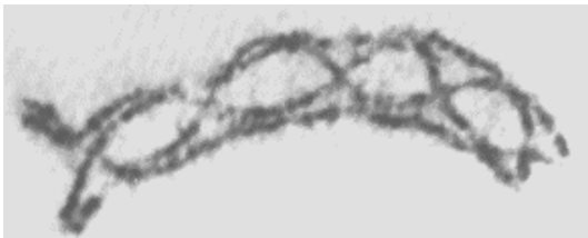
Five chiasmata in a tetrad of the grasshopper
